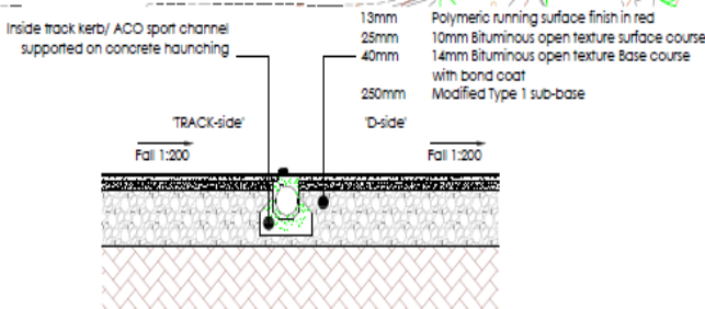
AA TYPICAL NEW POLYMERIC 'D' AREA SCALE: 1:20
