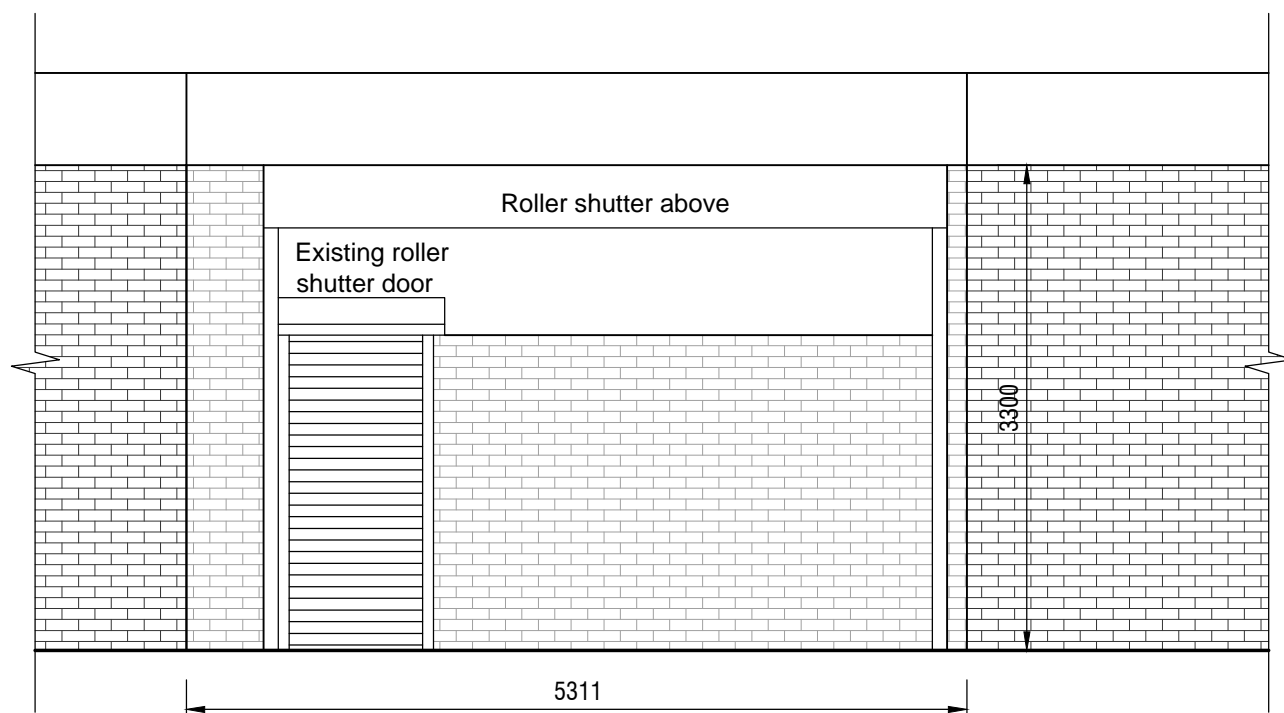
Elevation A As Existing Scale 1:50
