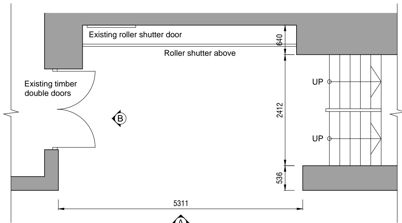
Floor Plan As Existing Scale 1:50
