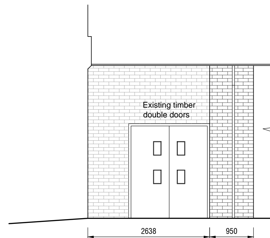
Elevation B As Existing Scale 1:50
