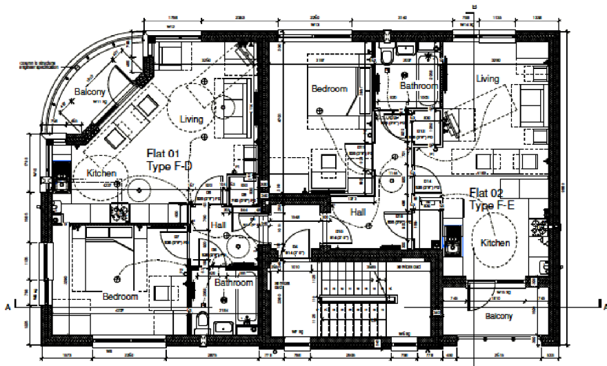
First Floor Plan 1:50
