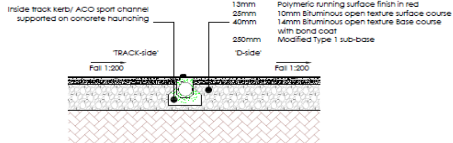
AA TYPICAL NEW POLYMERIC 'D' AREA SCALE 1:20
