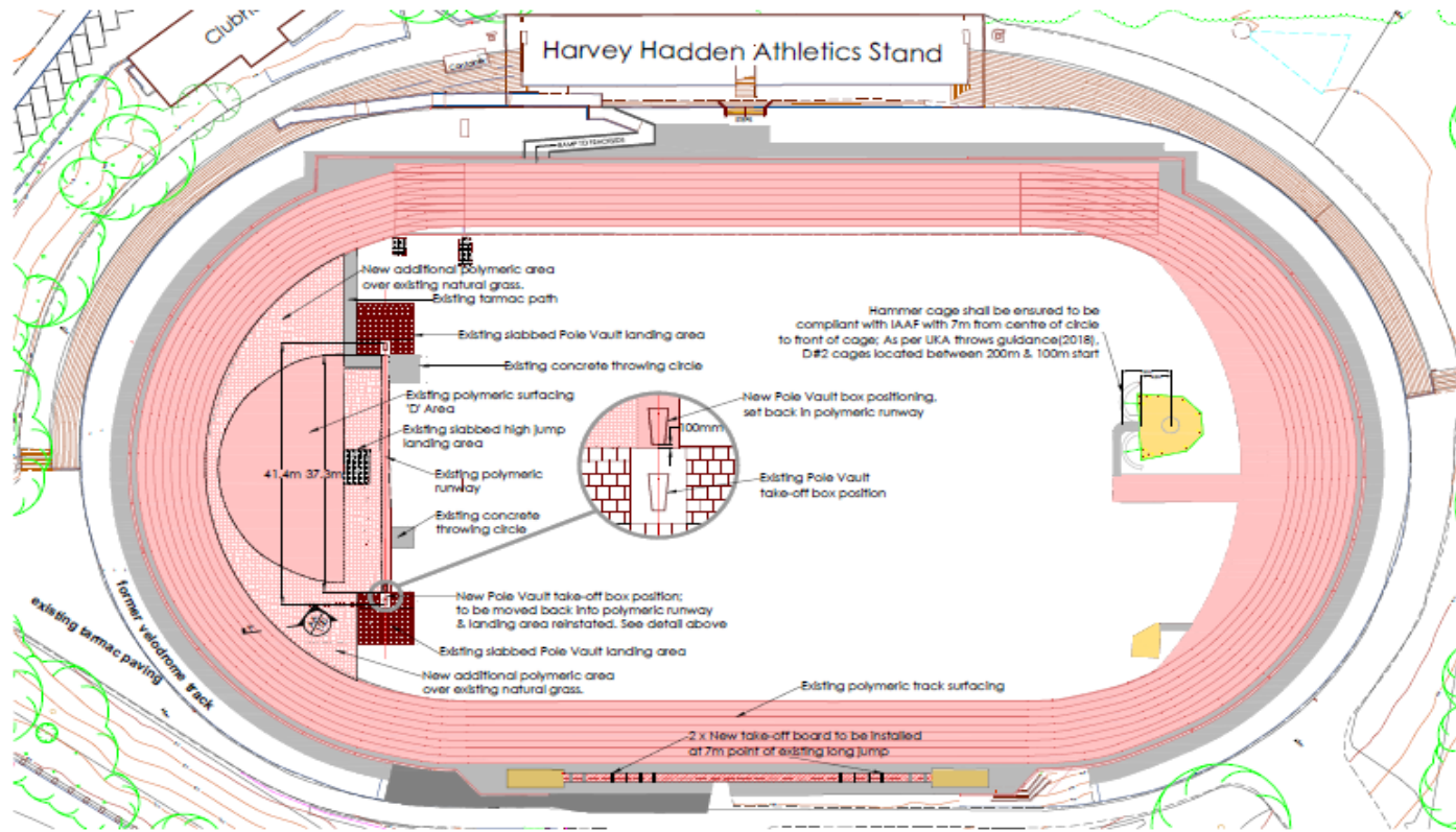
01 GENERAL ARRANGEMENT SCALE 1:750
